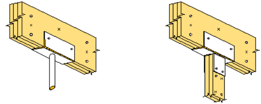
BEARING FOR SIMPLE OR CONTINUOUS BEAM SPAN
